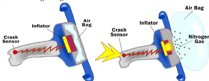
Figure 2 Functioning of Air Bag
