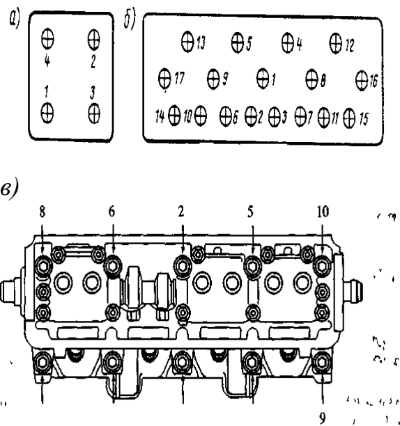
3-picture. Kamaz-740 (a), ZIL-130 (b) and Nexia (e) the sequence of tightening the cylinder head nuts of the engines.
