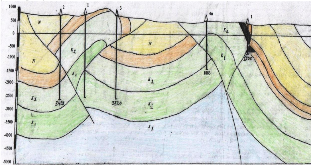
2- rasm. Shakarlik-Astana maydonining II chiziq bo'yicha geologik kesimi (A.A.Abidov bo'yicha, 1990 y)
