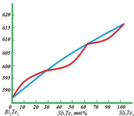
Figure 1. State diagram of \text{Bi}_2\text{Te}_3\text{-Sb}_2\text{Te}_3
