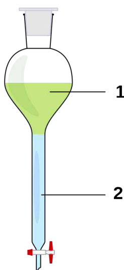
Figure 1. Schematic of a separatory funnel showing two immiscible liquids, where 1 is any phase less dense than 2. Phase 1 is typically an organic solvent and 2 an aqueous phase.
